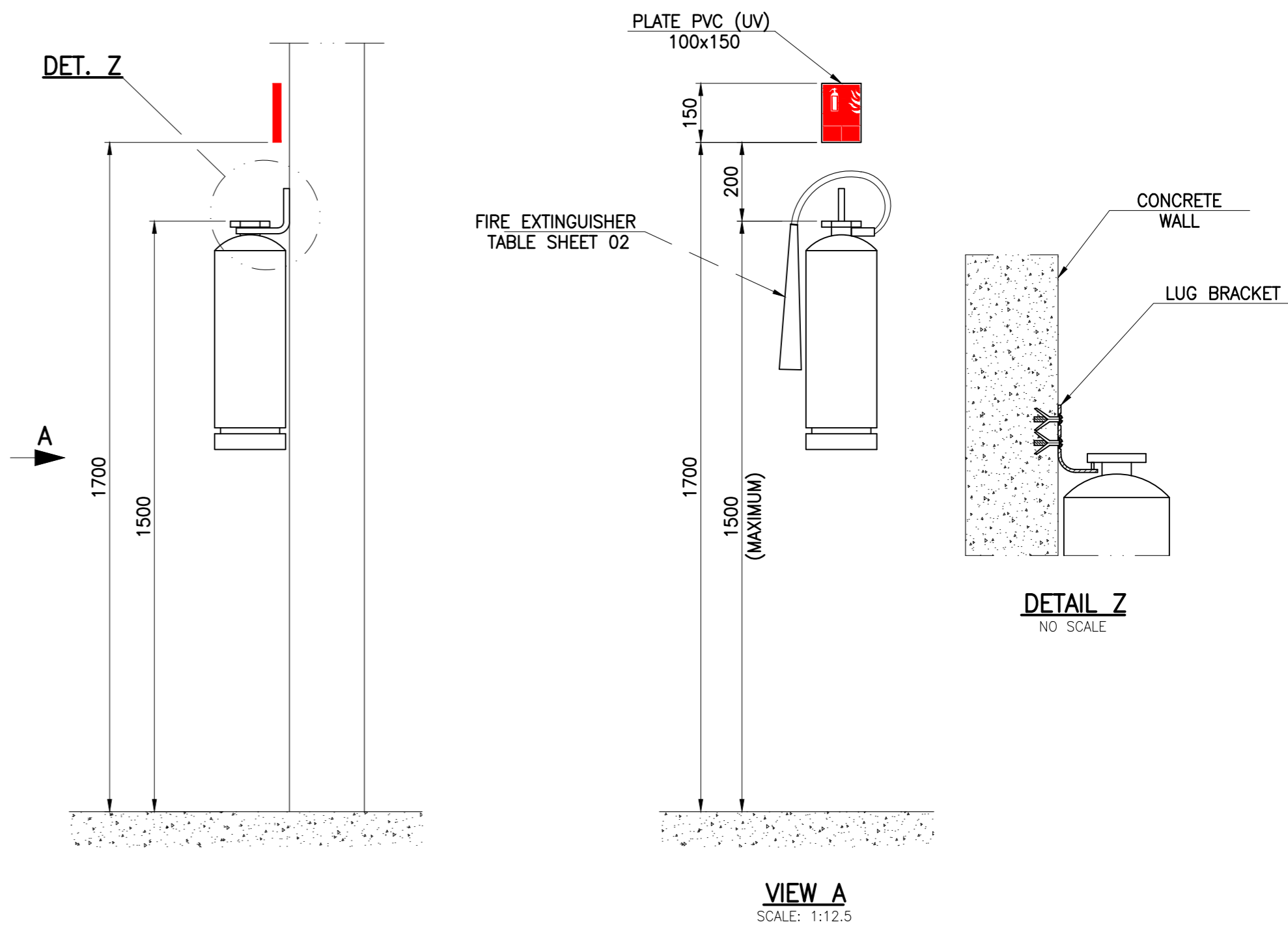
FIXATION 02 – SCHEME TO INDOOR AREAS (CONCRETE WALL) (13x)
