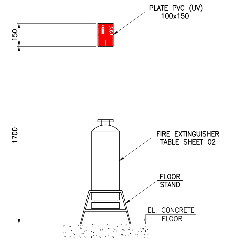
FIXATION 03 – SCHEME TO FLOOR SUPPORT (8x)
