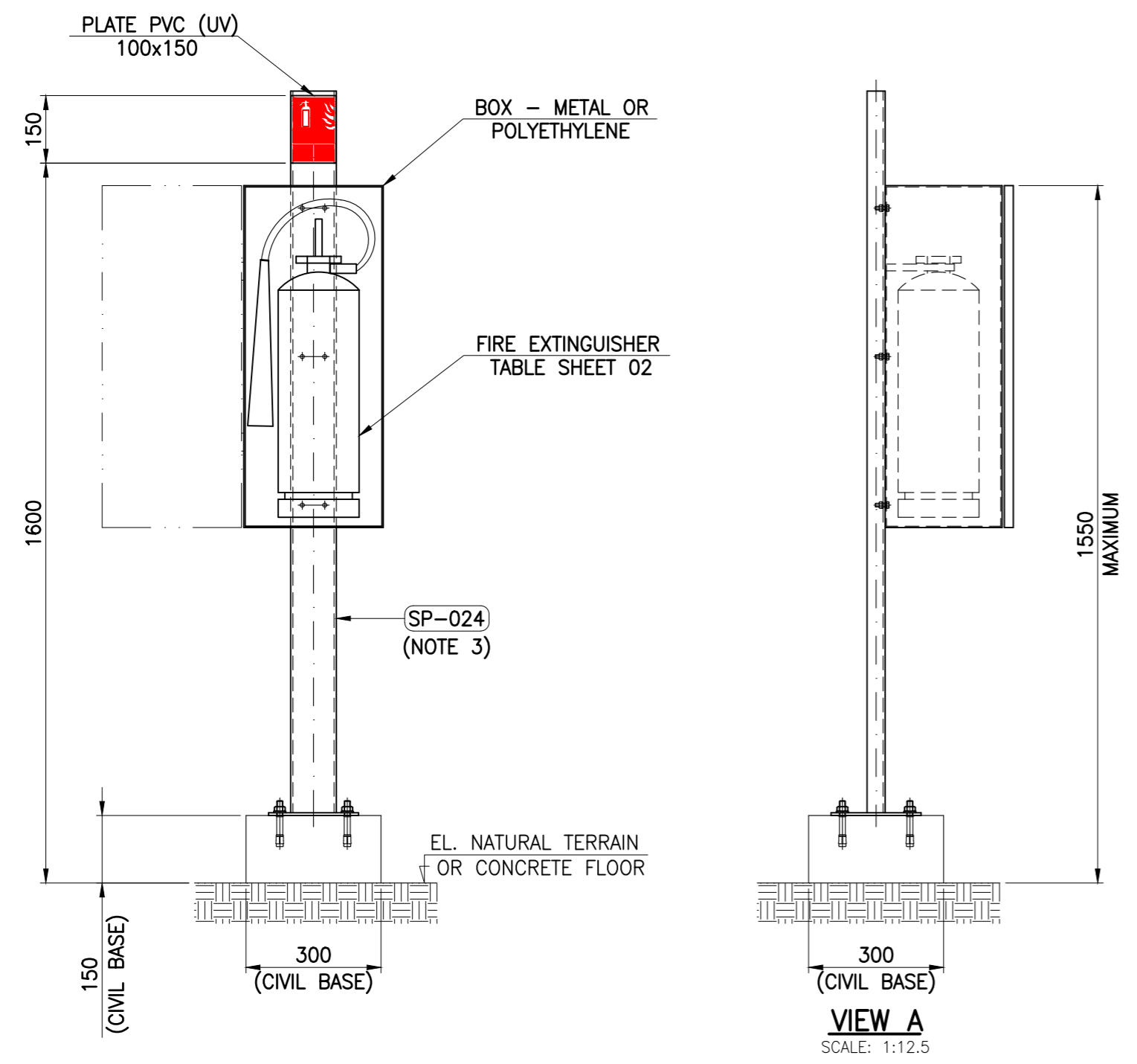
FIXATION 01 – SCHEME TO OUTDOOR AREAS (14x)
